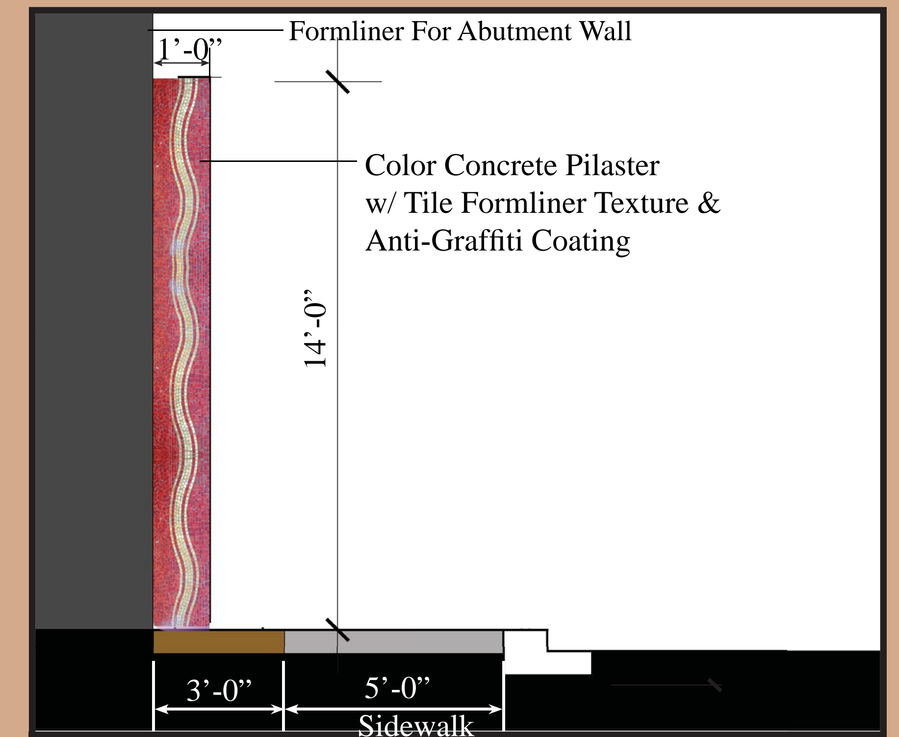
Concrete Pilaster
