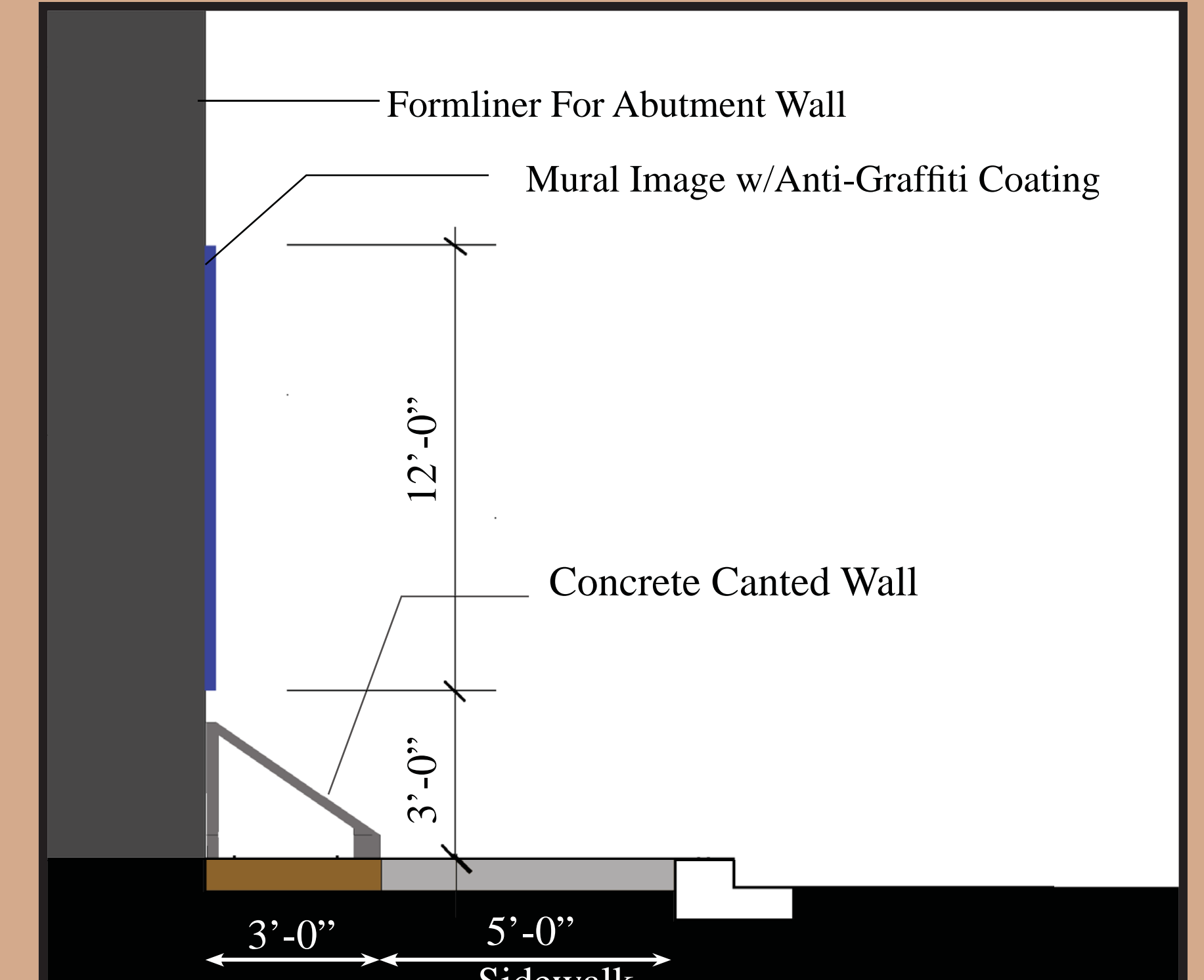
Panel Section
